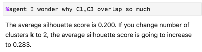
Fig. 4: Example of a conversation with an agent for a clustering problem. The user—gray boxes—addresses the agent by explicitly requesting a command and also conveying doubt about the results. The agent, in addition to answering the question, also proactively makes suggestions to the user. In this example, the explanation about a validation metric—silhouette scores—is provided verbally.
